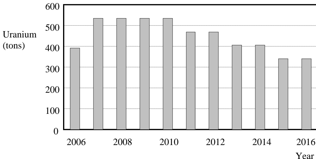
Figure 8: Estimated annual domestic uranium requirements for unsafeguarded heavy water power reactors. 78
